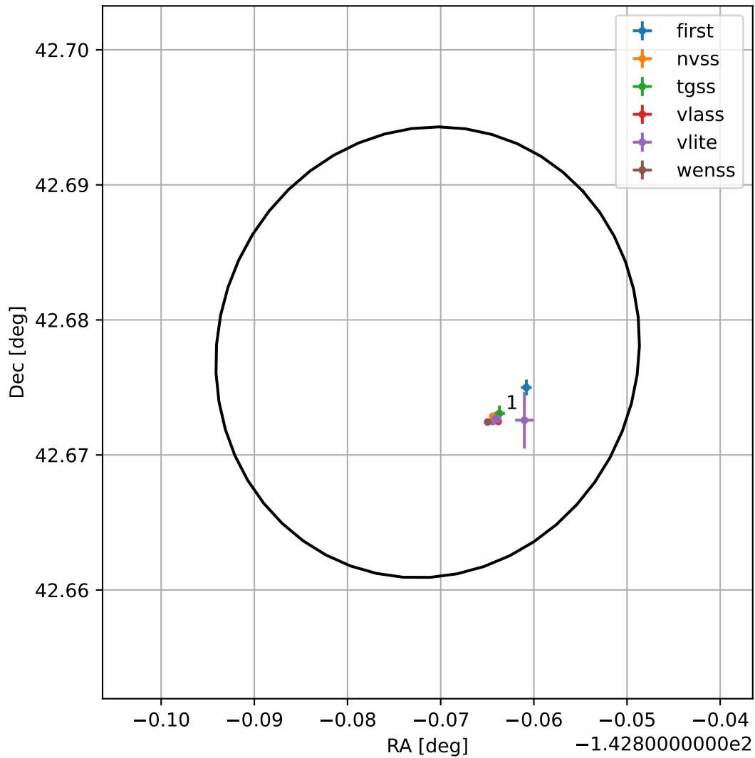
4FGL J1428.5+4240
