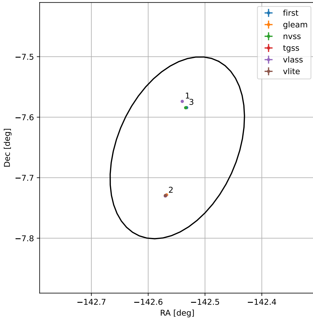
4FGL J1429.8-0739
