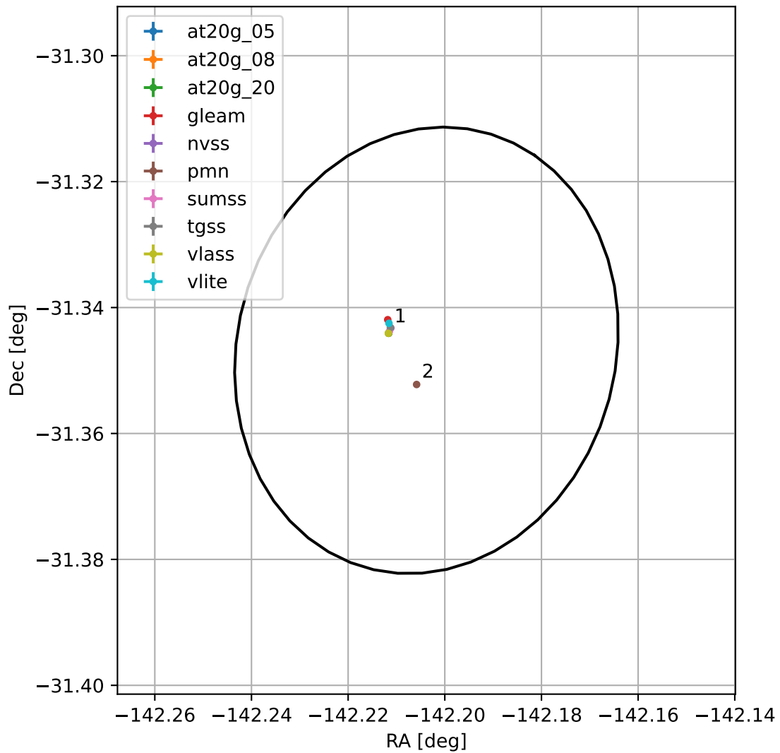
4FGL J1431.1-3120
