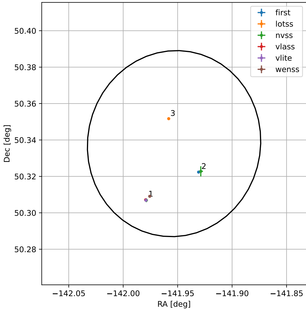
4FGL J1432.1+5020
