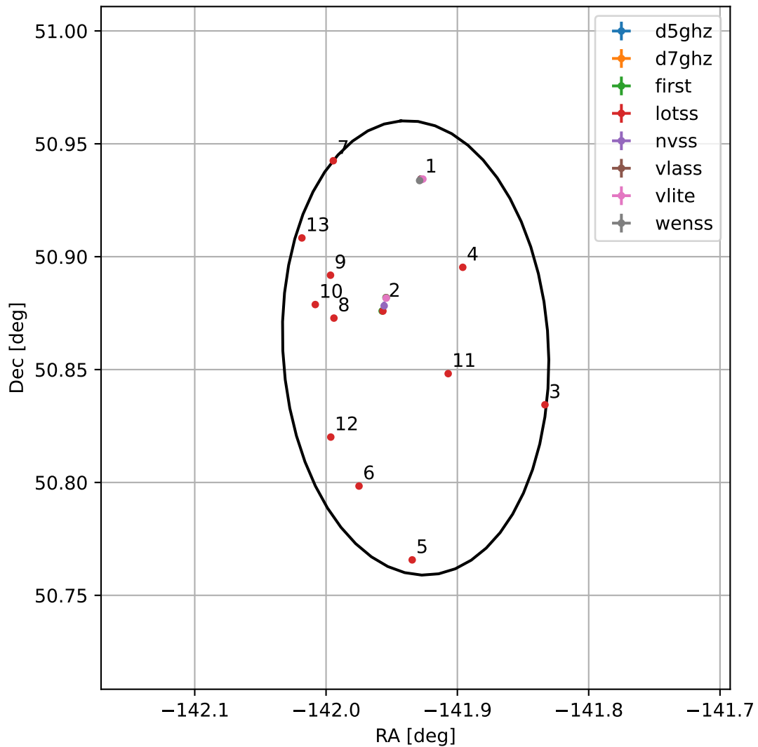
4FGL J1432.2+5051
