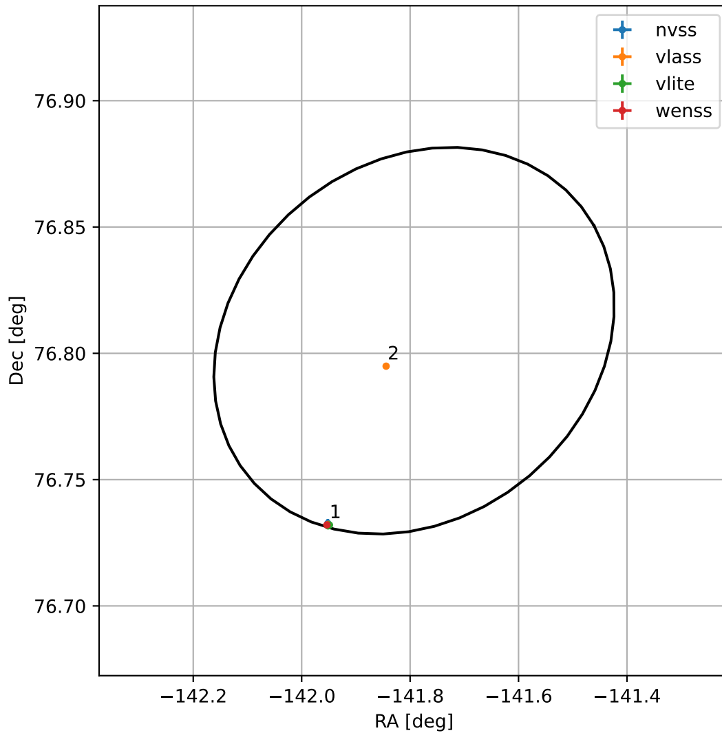
4FGL J1432.8+7648
