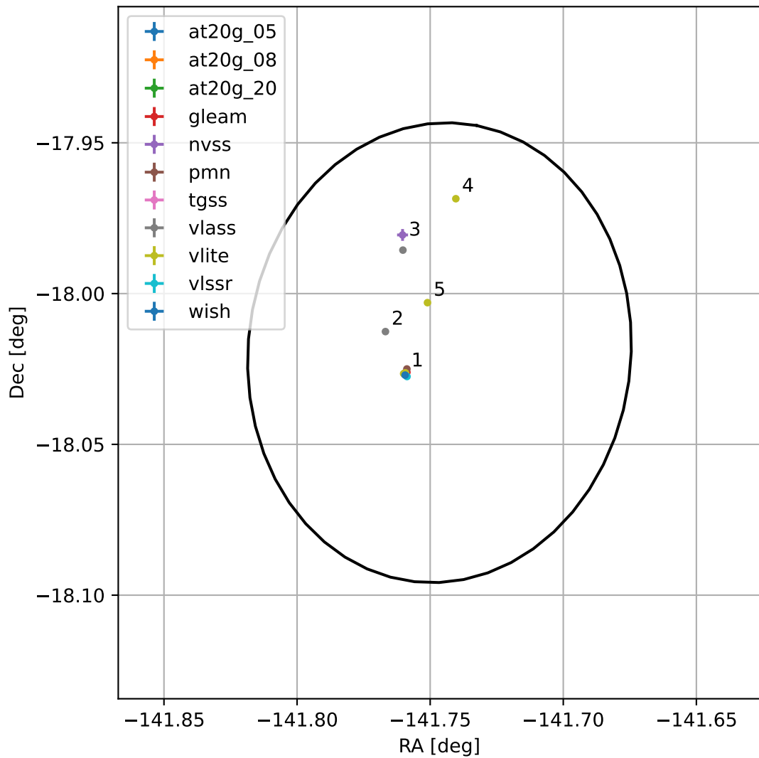
4FGL J1433.0-1801
