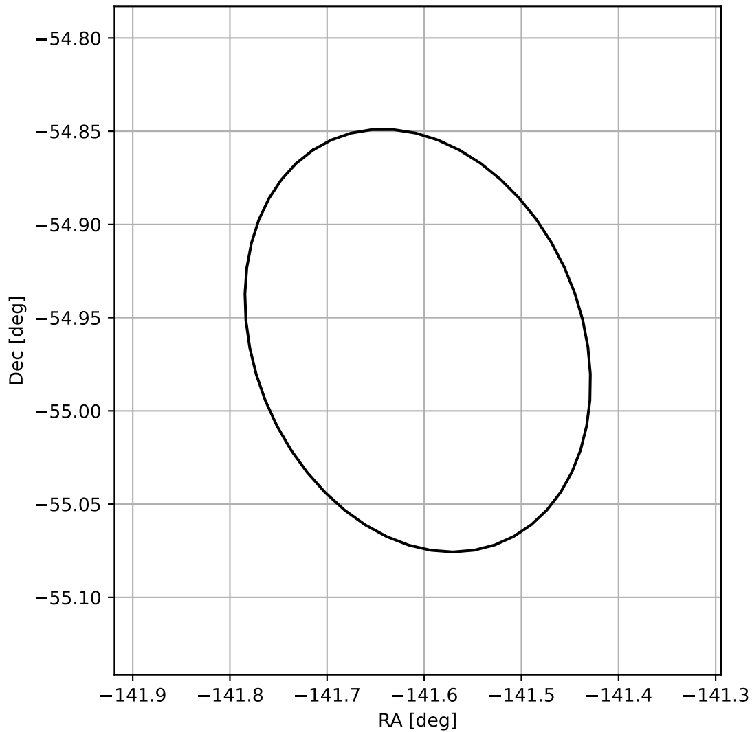
4FGL J1433.5-5457
