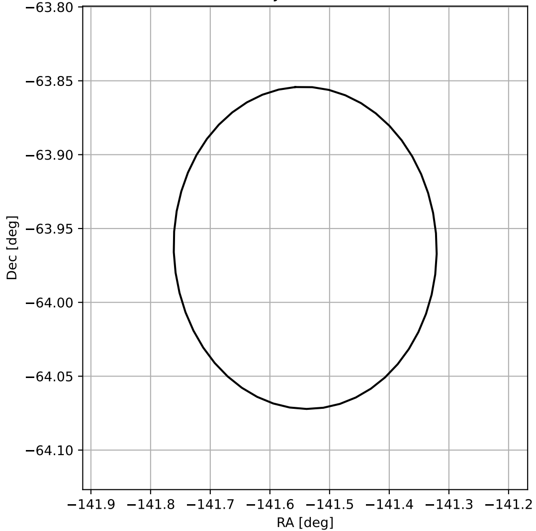
4FGL J1433.8-6357
