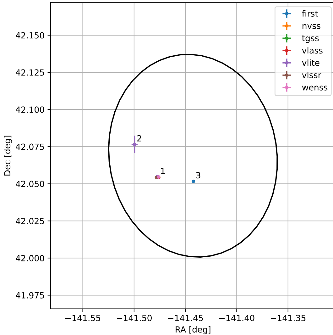
4FGL J1434.2+4204
