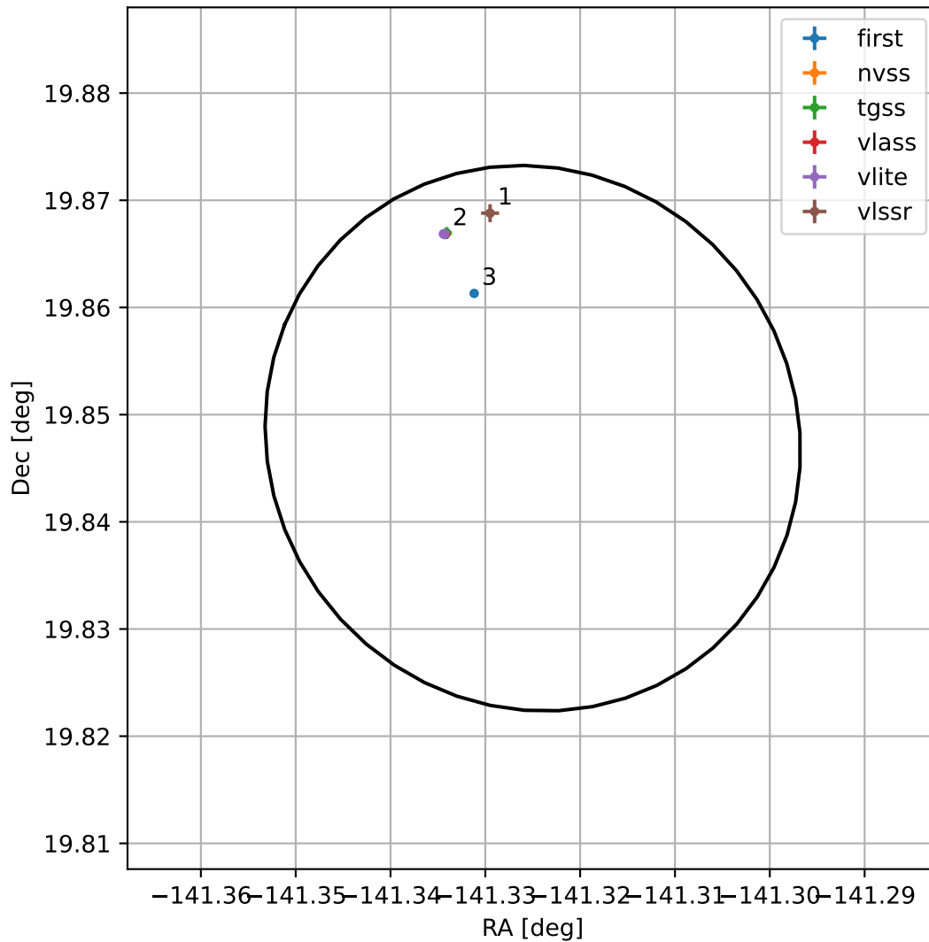
4FGL J1434.7+1950
