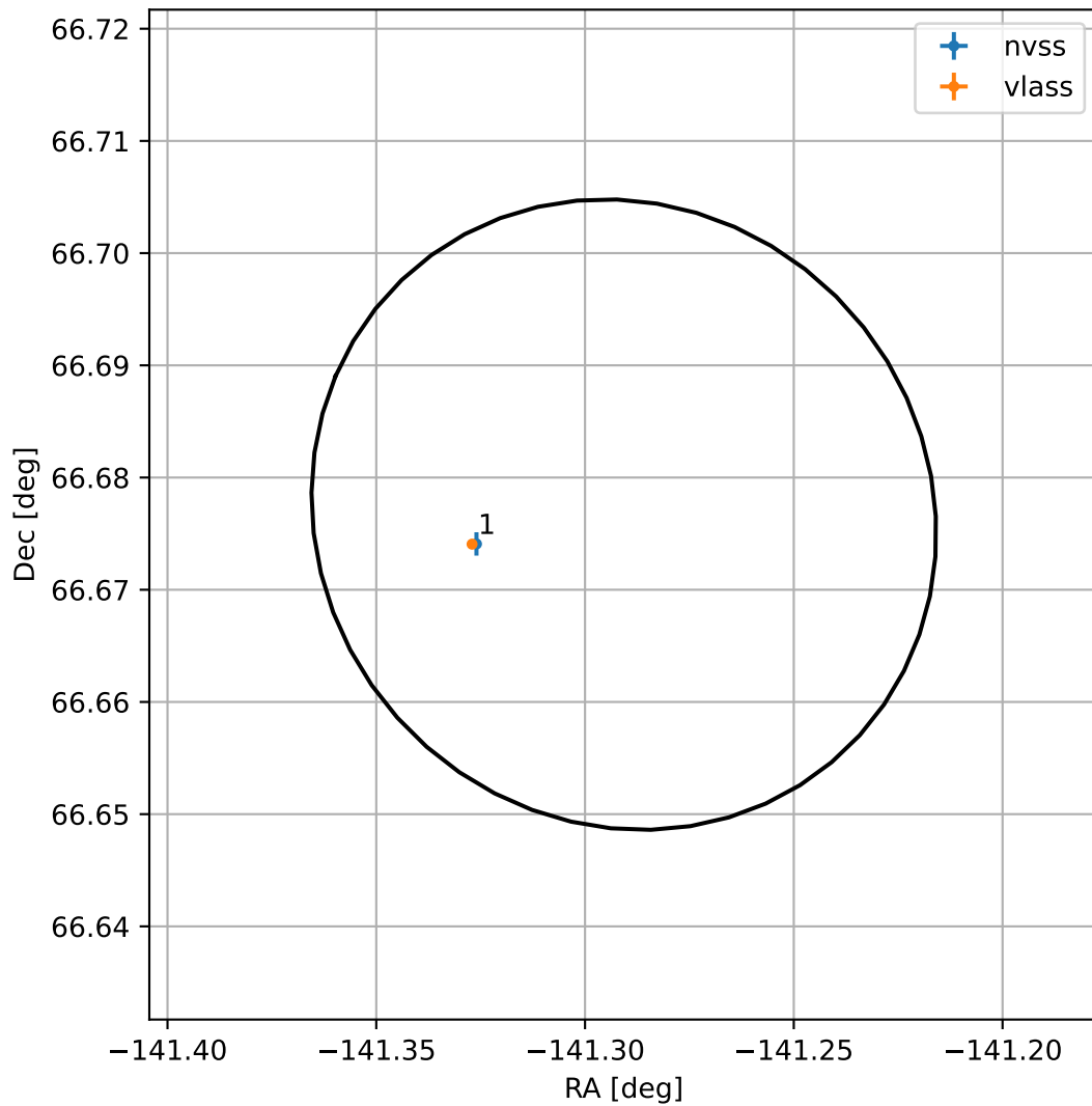
4FGL J1434.8+6640
