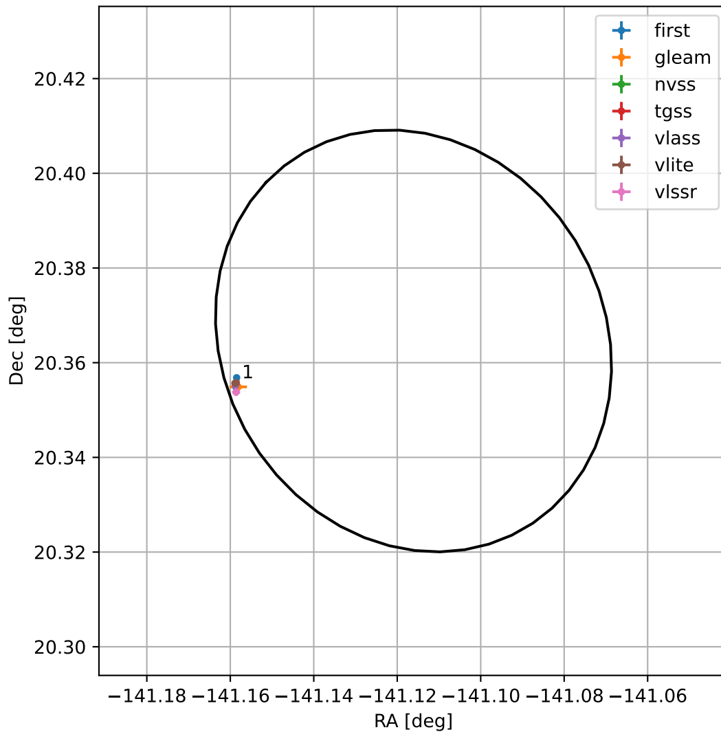
4FGL J1435.5+2021
