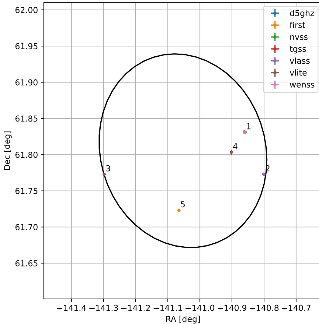
4FGL J1435.7+6148
