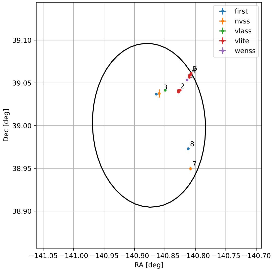
4FGL J1436.4+3900
