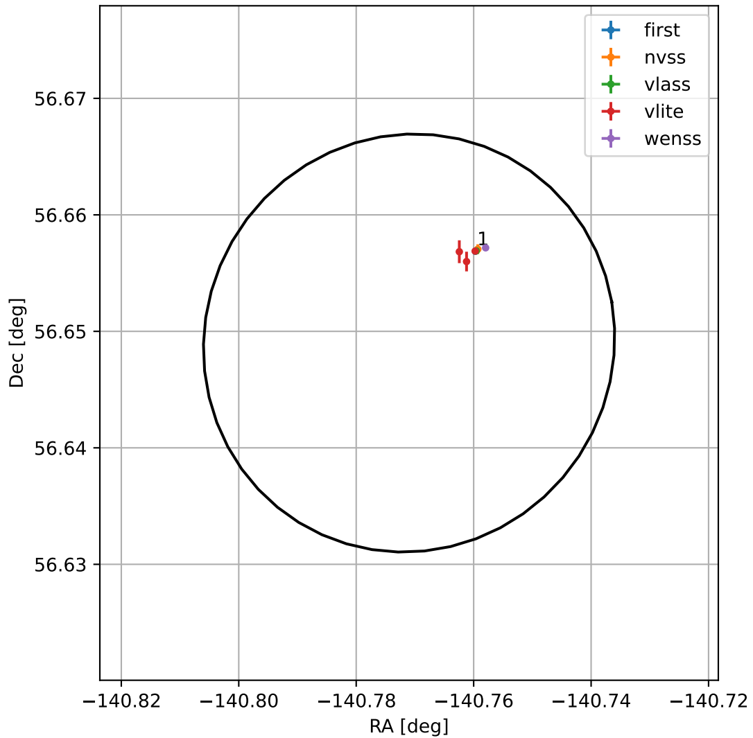
4FGL J1436.9+5638
