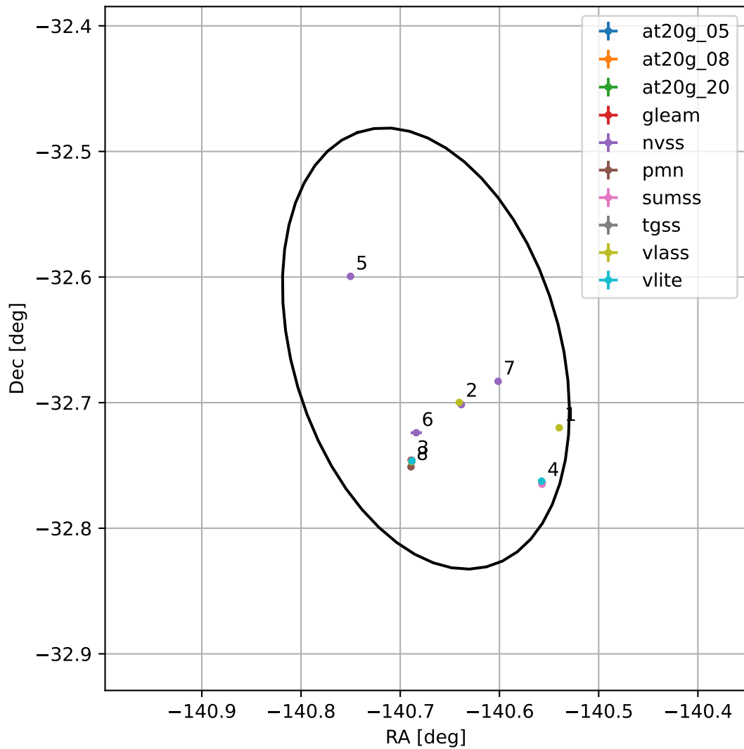
4FGL J1437.3-3239
