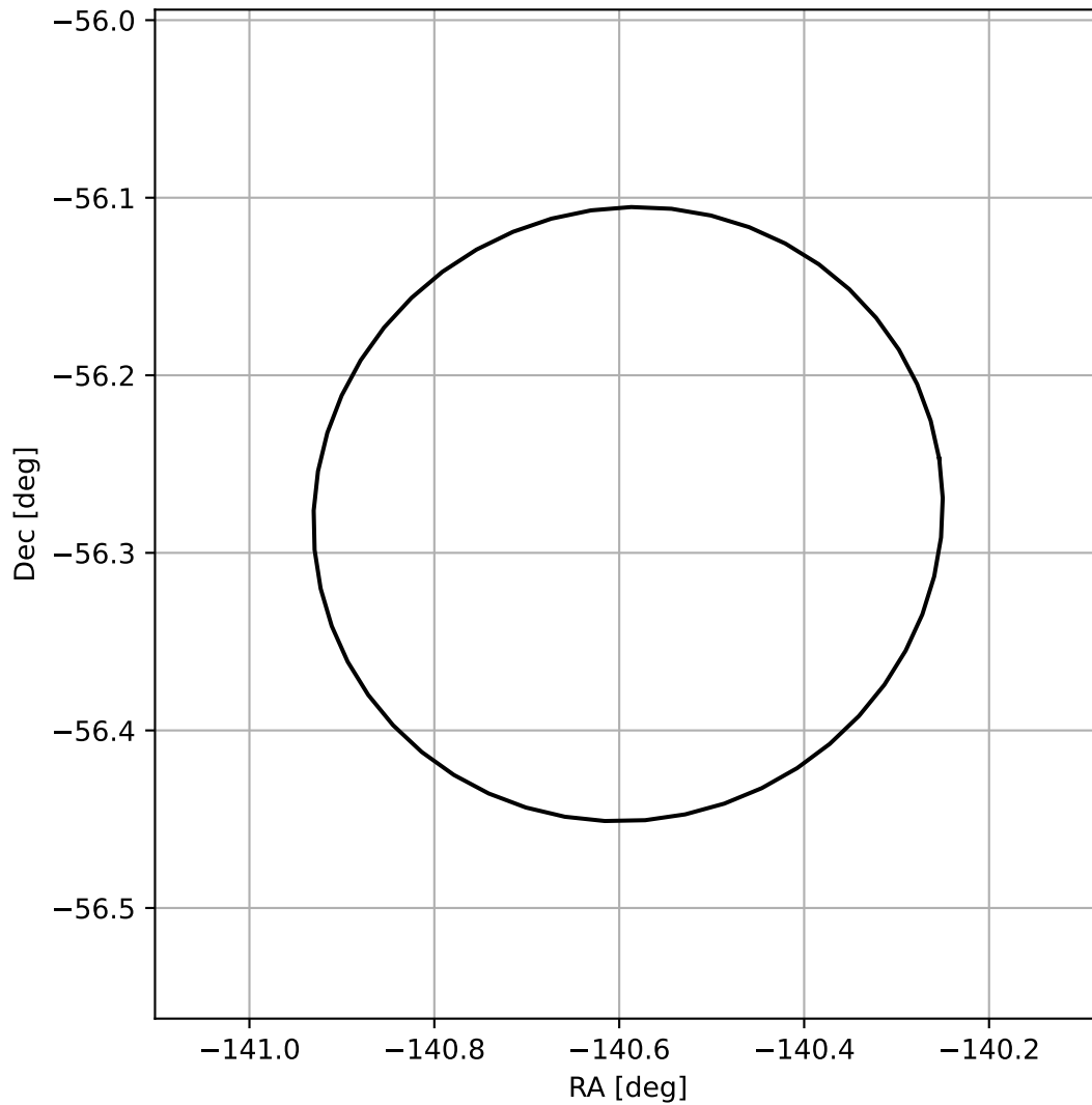
4FGL J1437.6-5616
