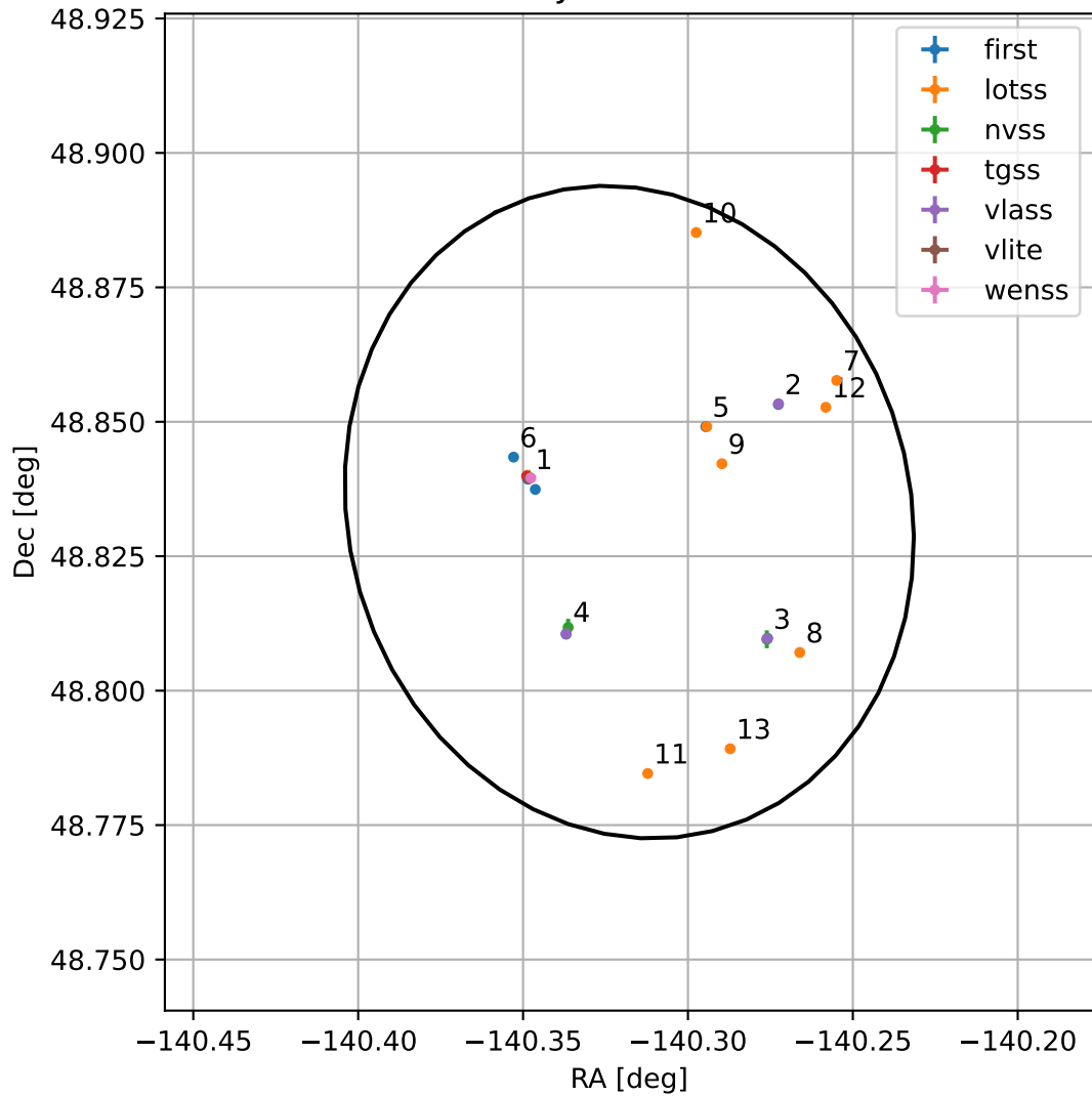
4FGL J1438.7+4849
