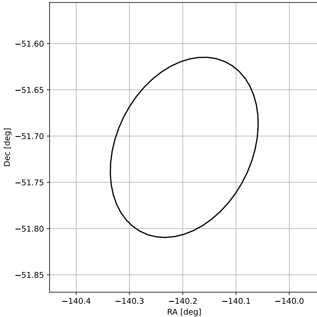
4FGL J1439.2-5142
