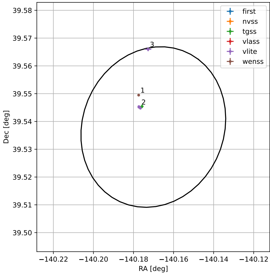
4FGL J1439.3+3932
