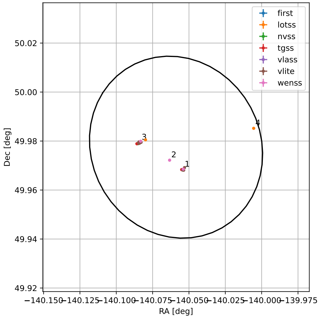
4FGL J1439.7+4958
