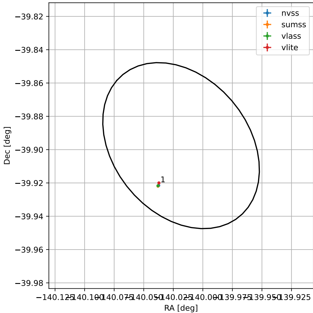
4FGL J1439.9-3953
