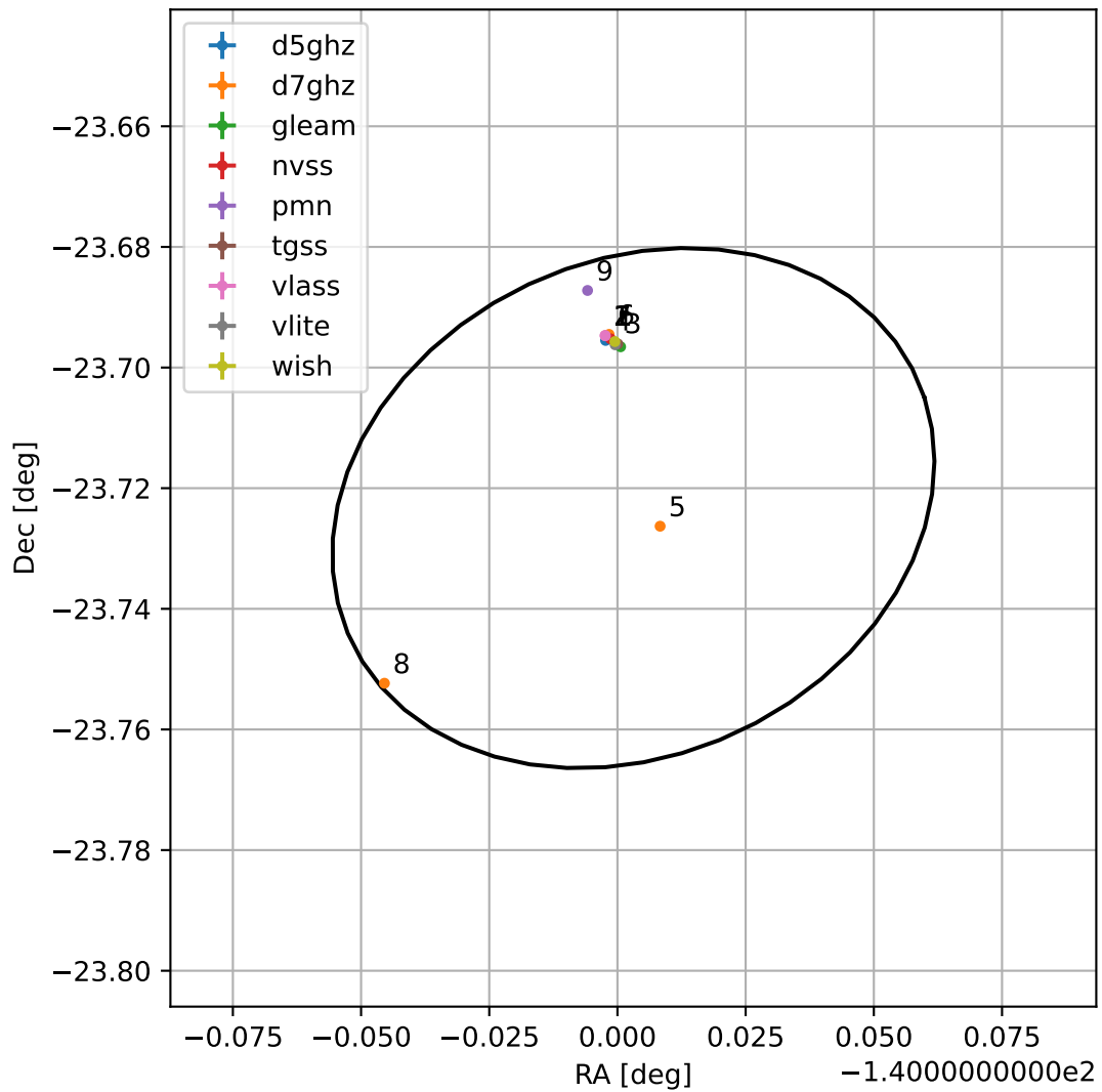
4FGL J1440.0-2343
