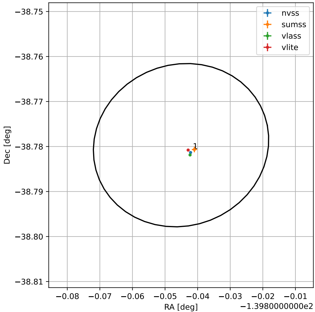
4FGL J1440.6-3846
