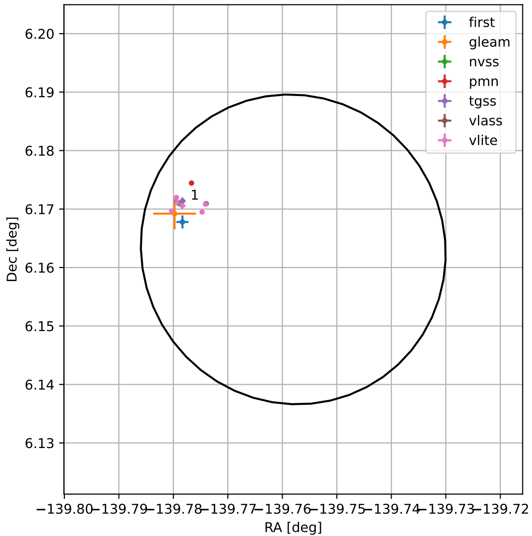
4FGL J1440.9+0609
