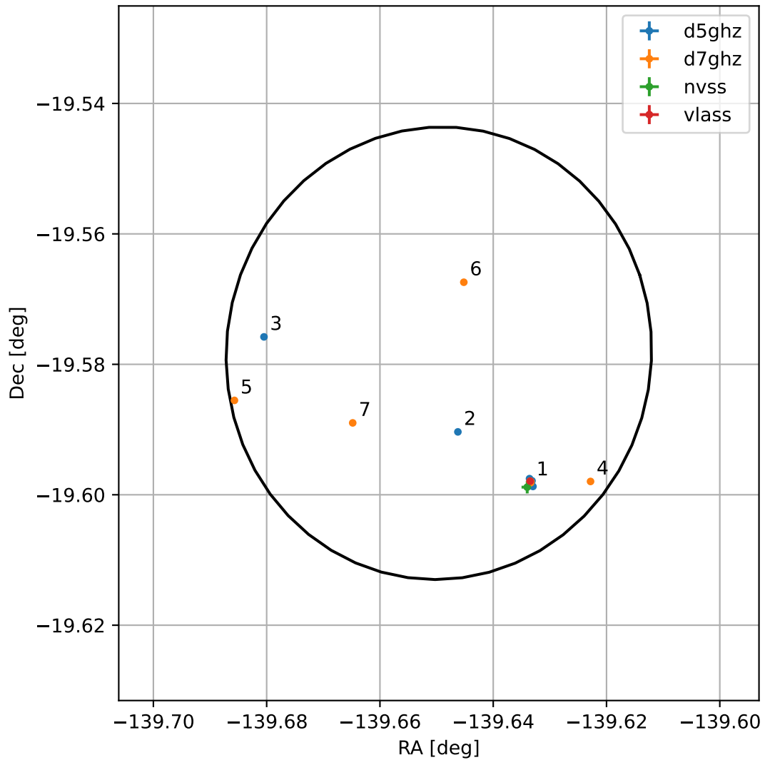
4FGL J1441.4-1934
