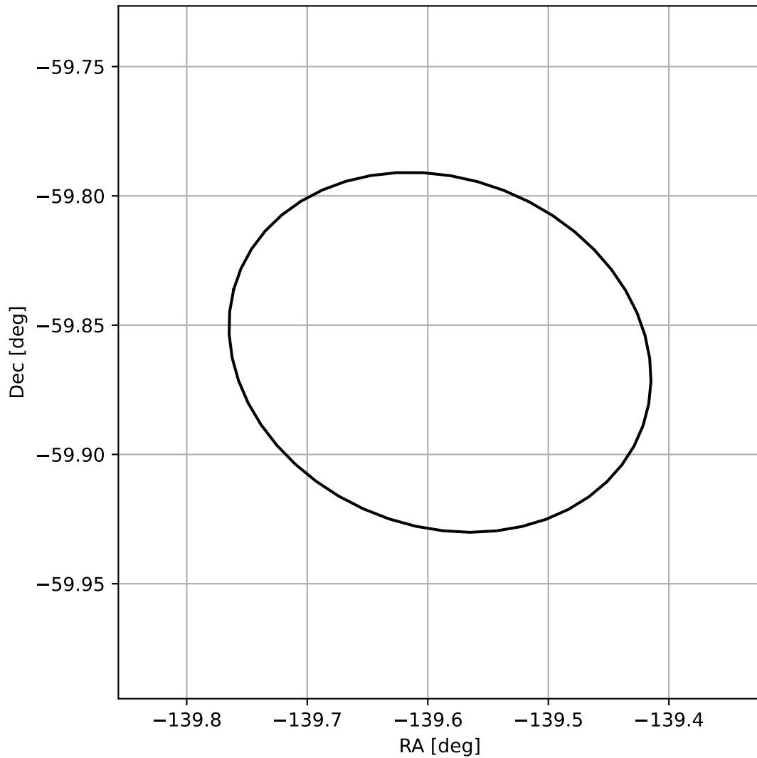
4FGL J1441.6-5951
