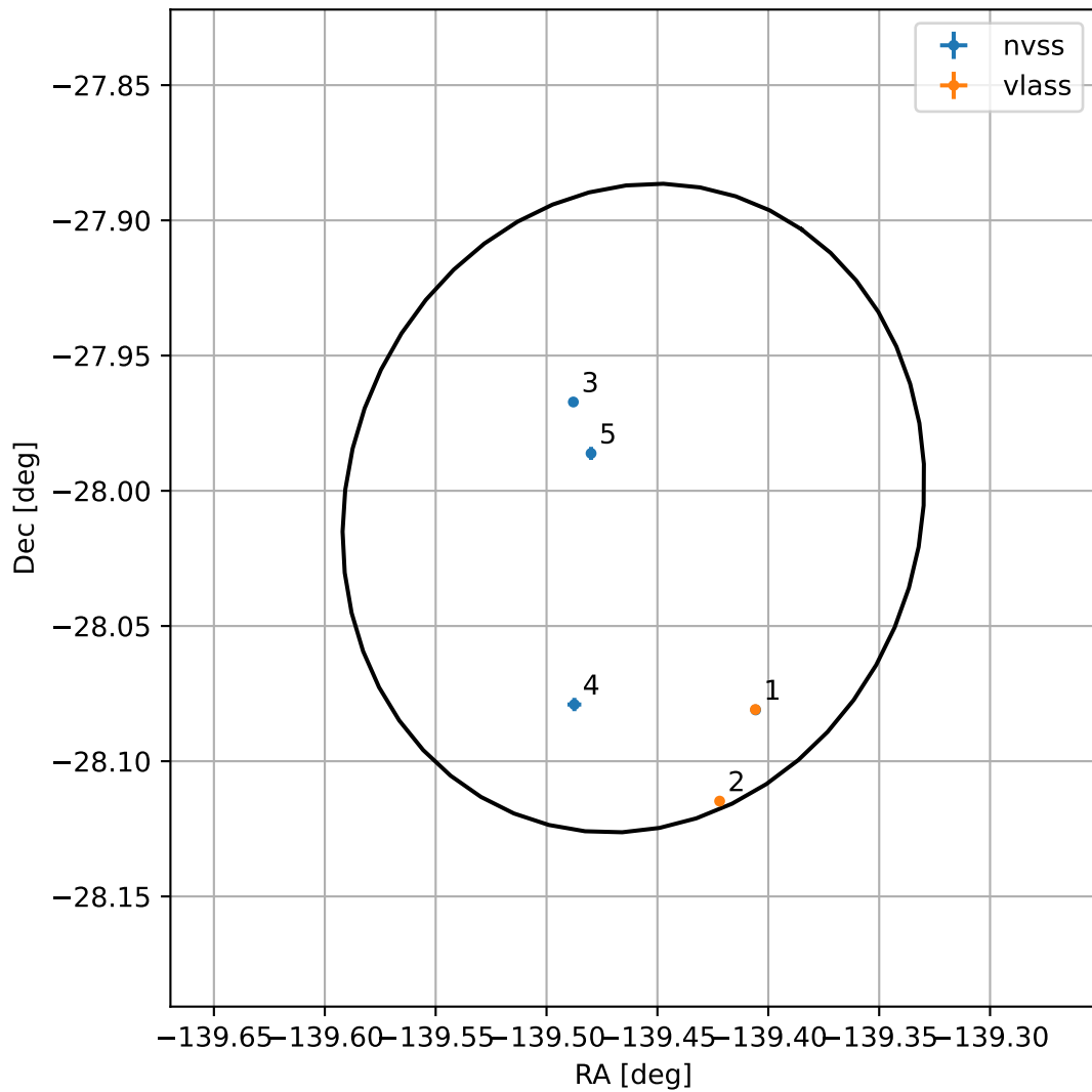
4FGL J1442.1-2800
