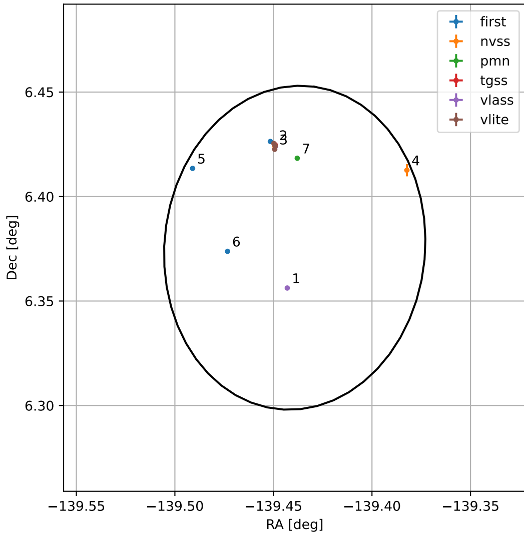
4FGL J1442.2+0622
