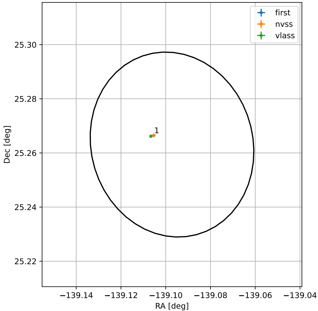
4FGL J1443.6+2515
