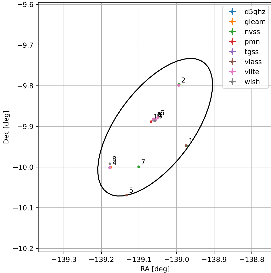
4FGL J1443.7-0954
