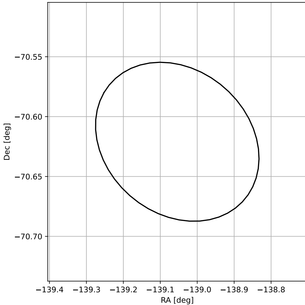
4FGL J1443.7-7037
