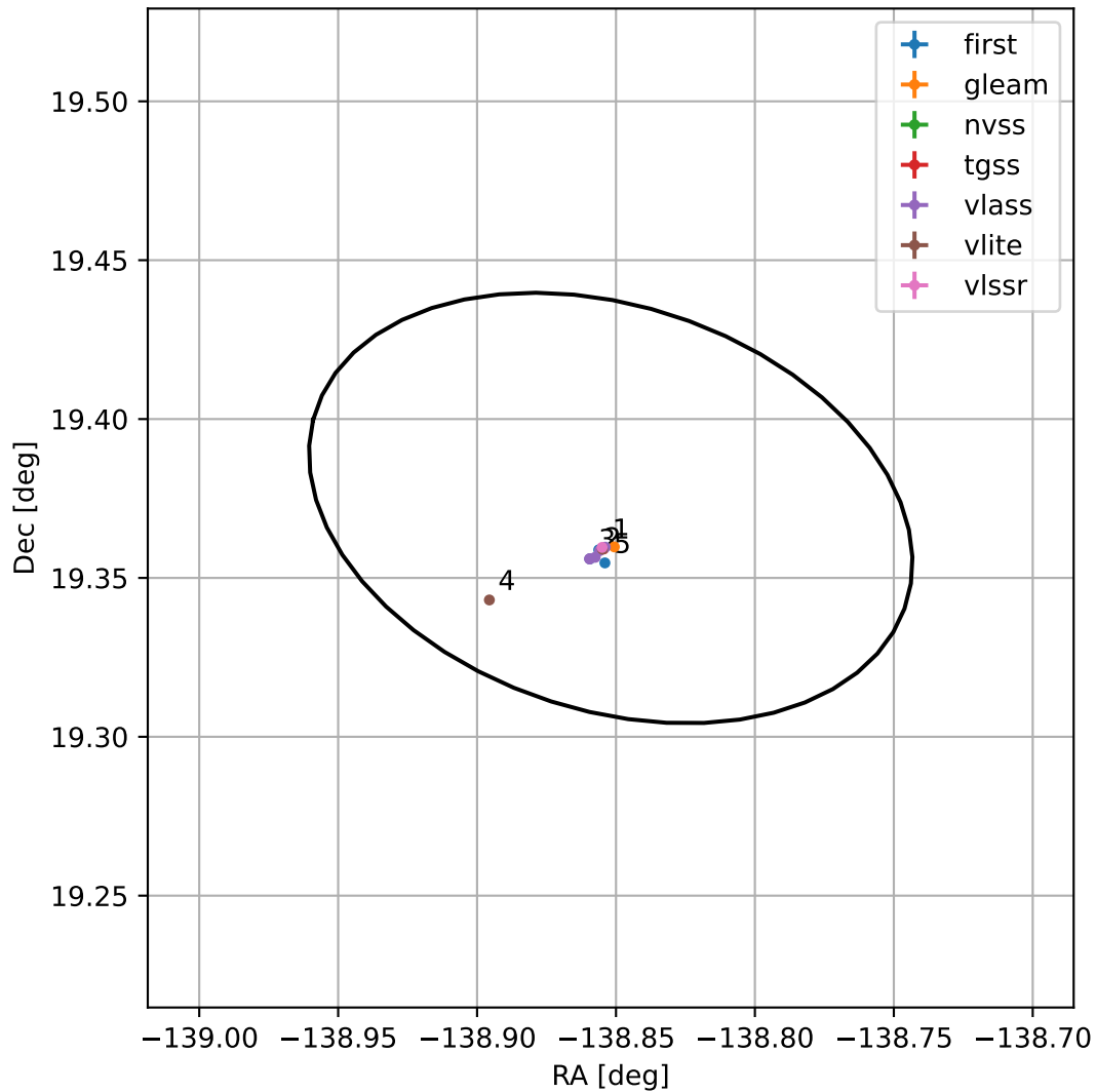
4FGL J1444.5+1922
