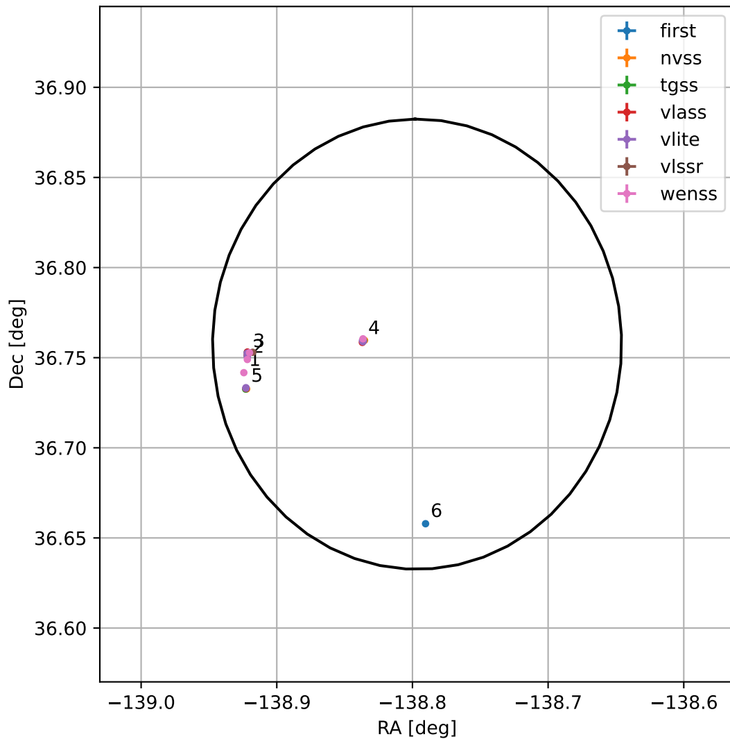
4FGL J1444.8+3645
