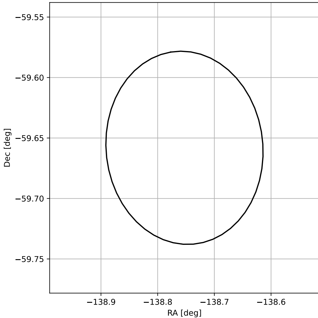
4FGL J1444.9-5939
