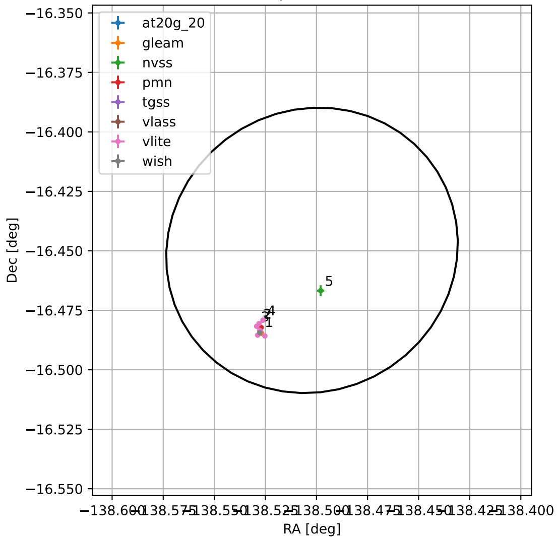
4FGL J1445.9-1626
