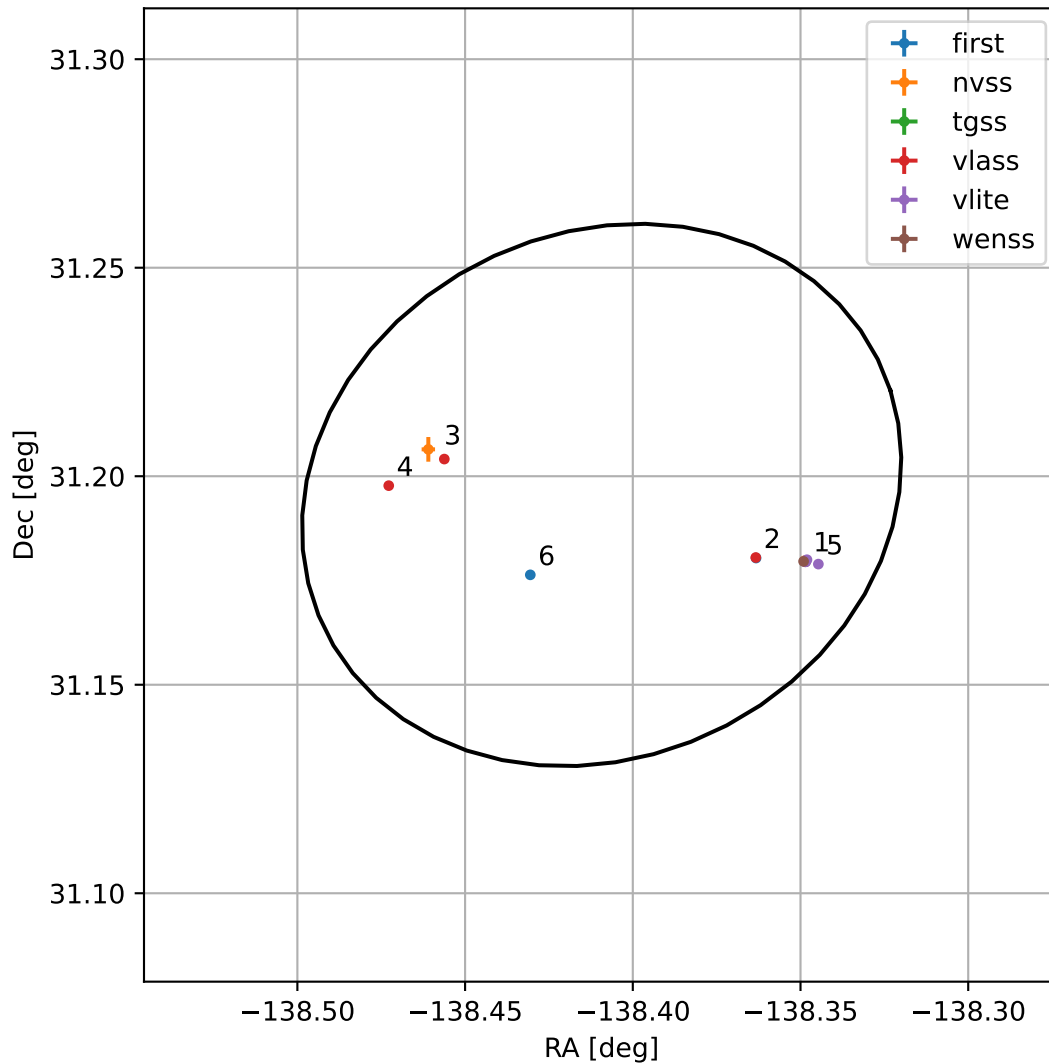
4FGL J1446.3+3111
