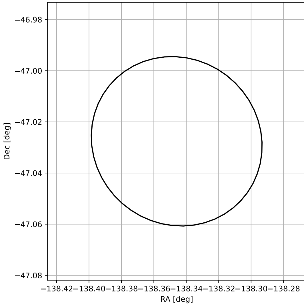
4FGL J1446.6-4701
