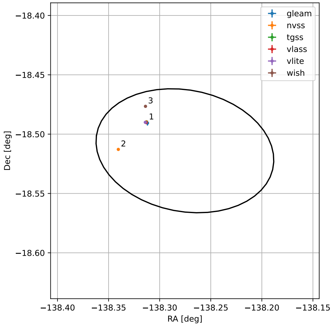
4FGL J1446.8-1830
