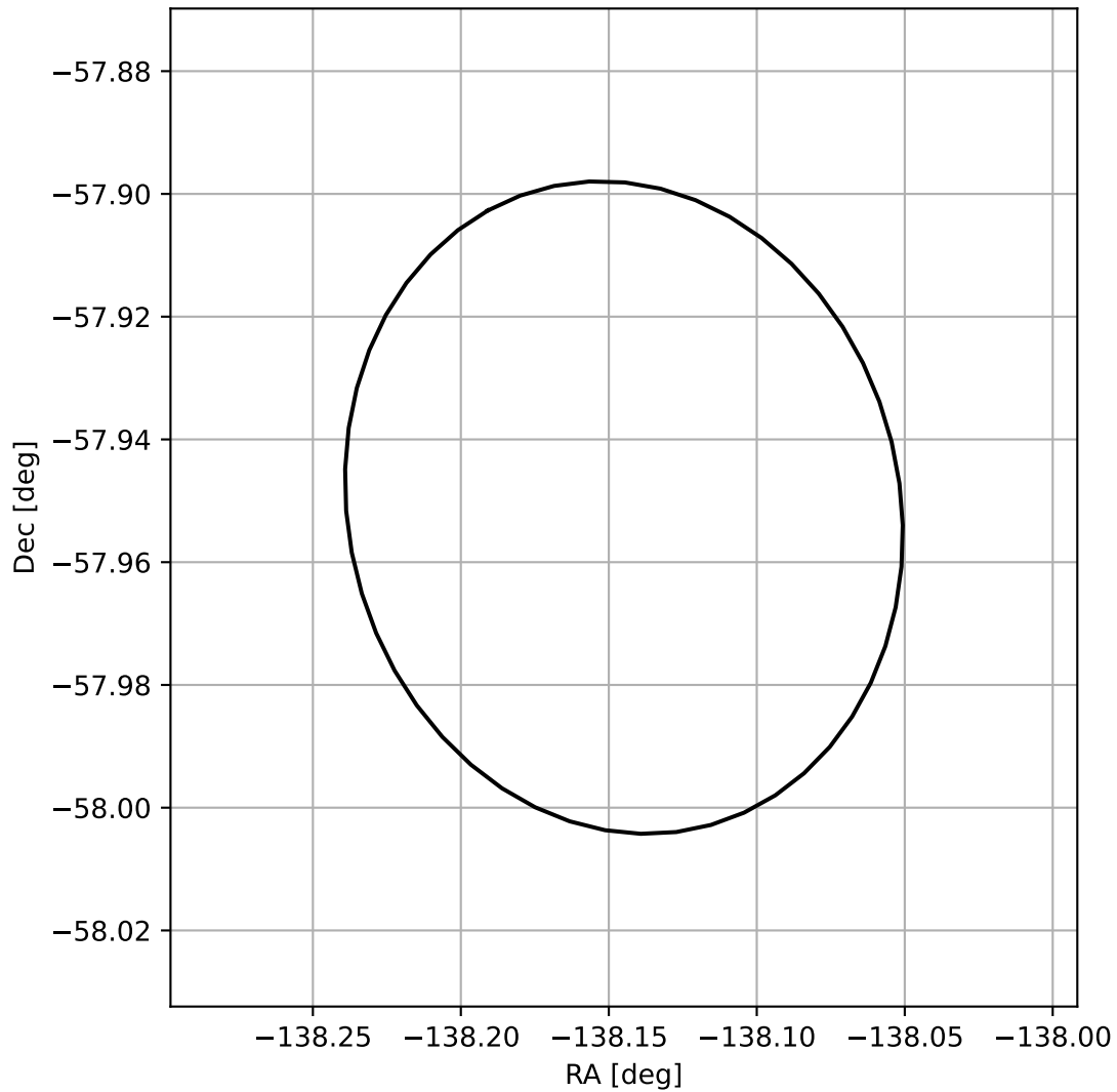
4FGL J1447.4-5757
