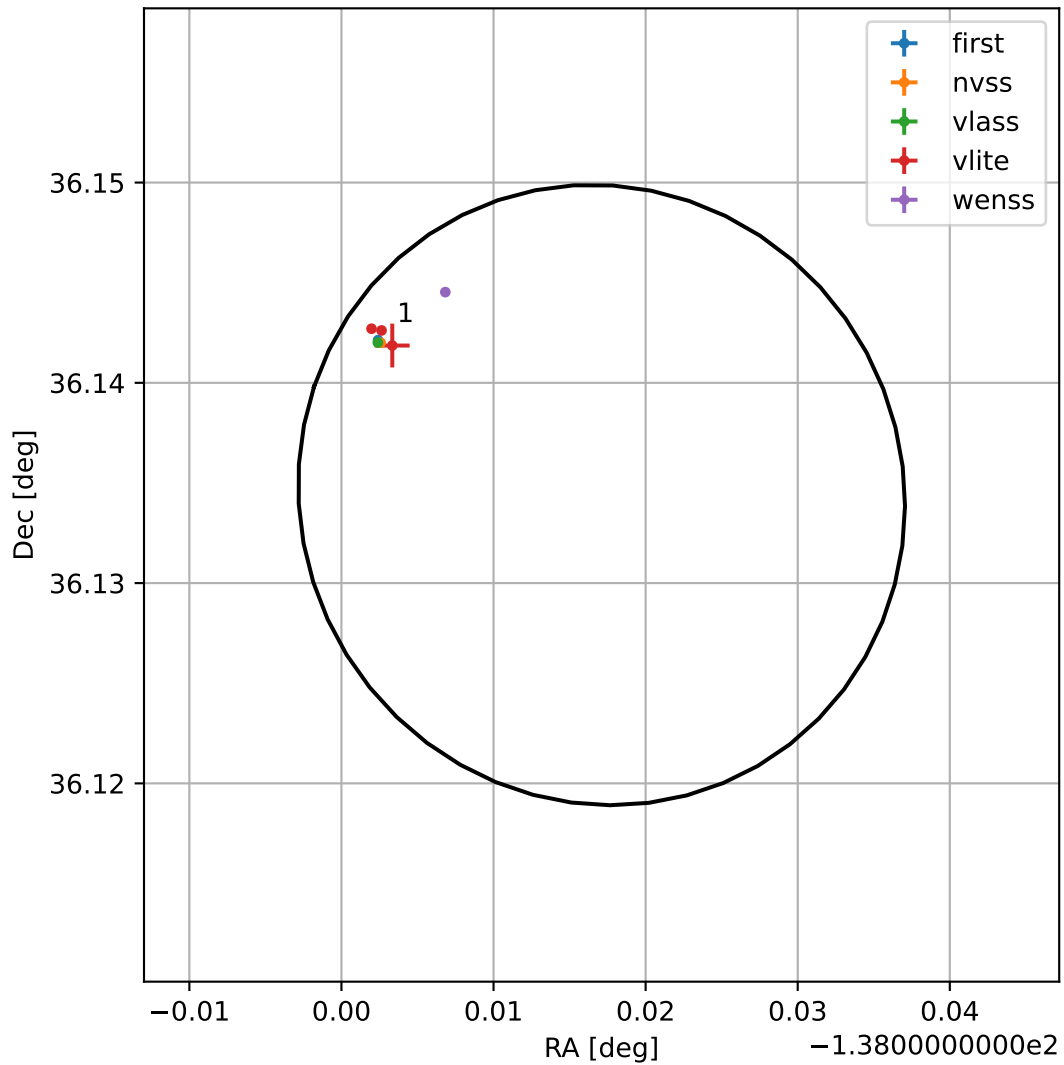
4FGL J1448.0+3608
