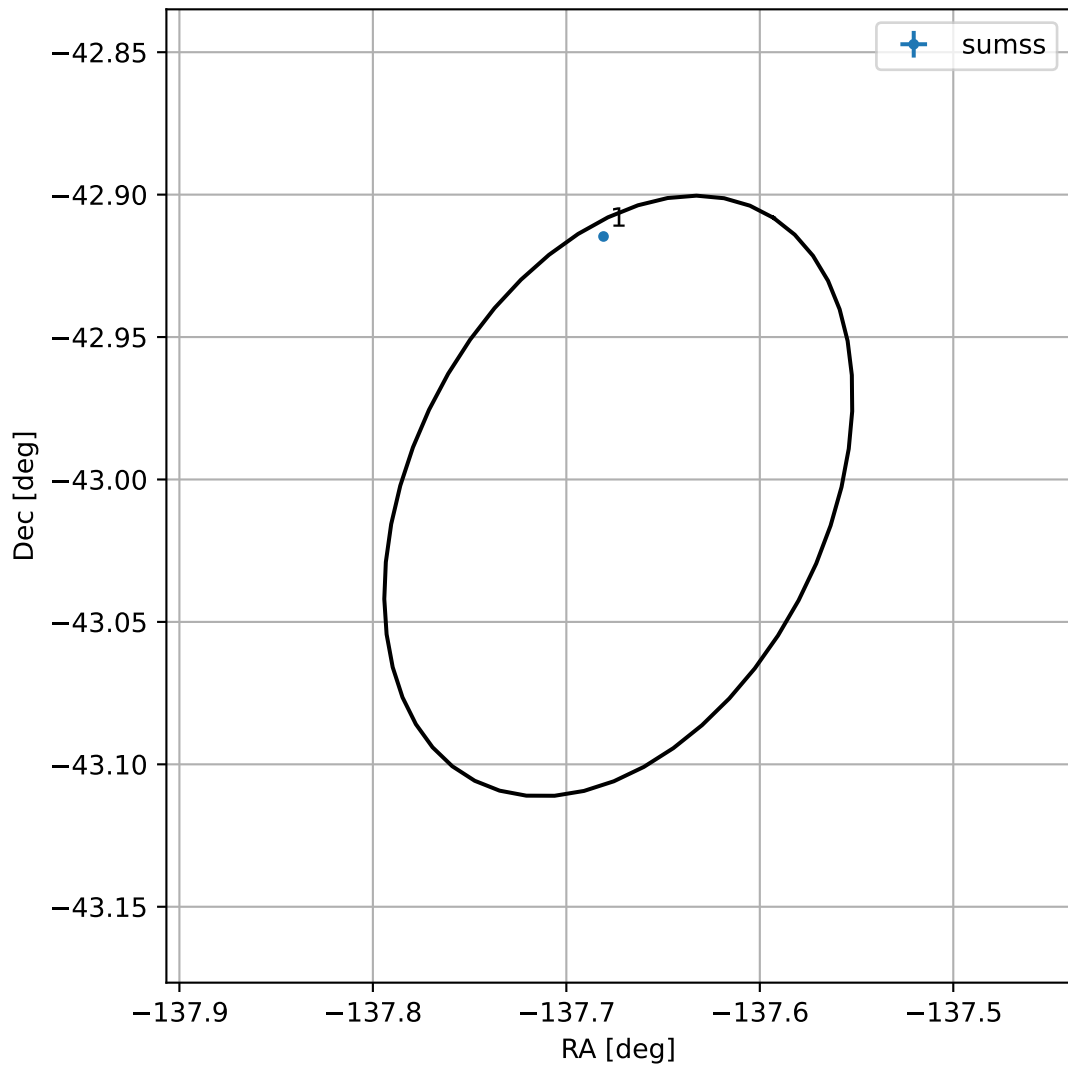
4FGL J1449.3-4300
