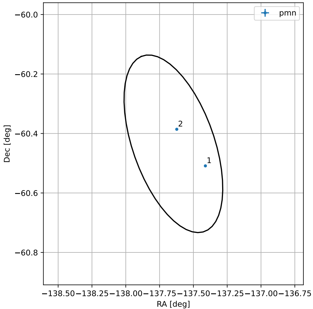
4FGL J1449.4-6026
