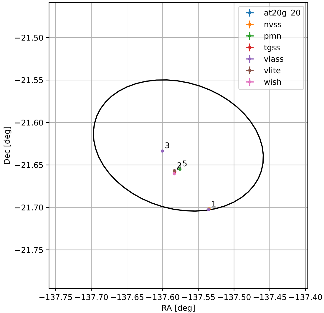
4FGL J1449.6-2137
