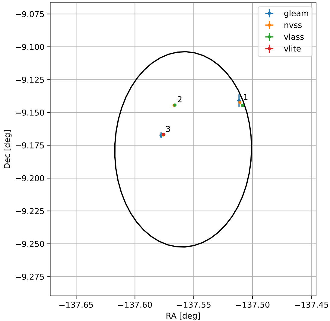
4FGL J1449.7-0910
