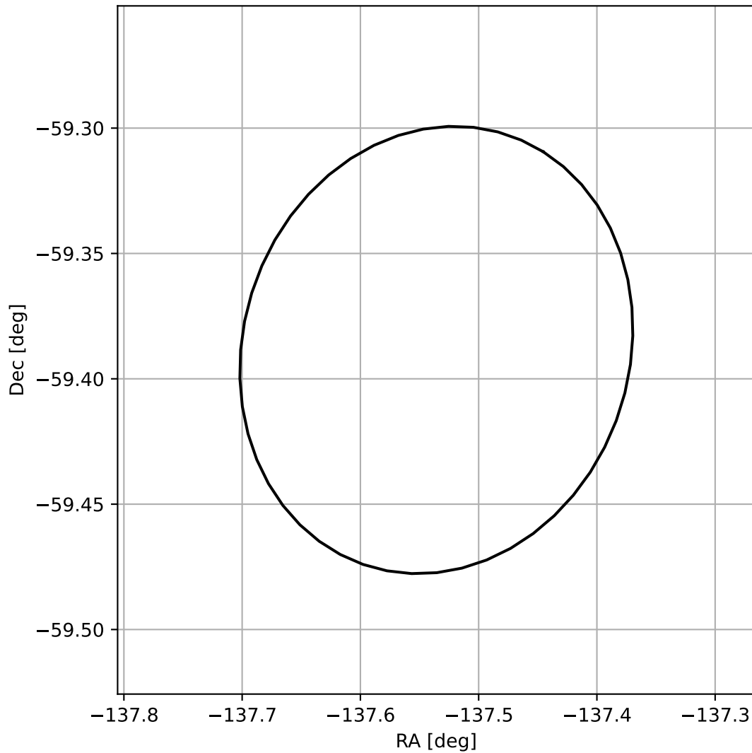
4FGL J1449.8-5923
