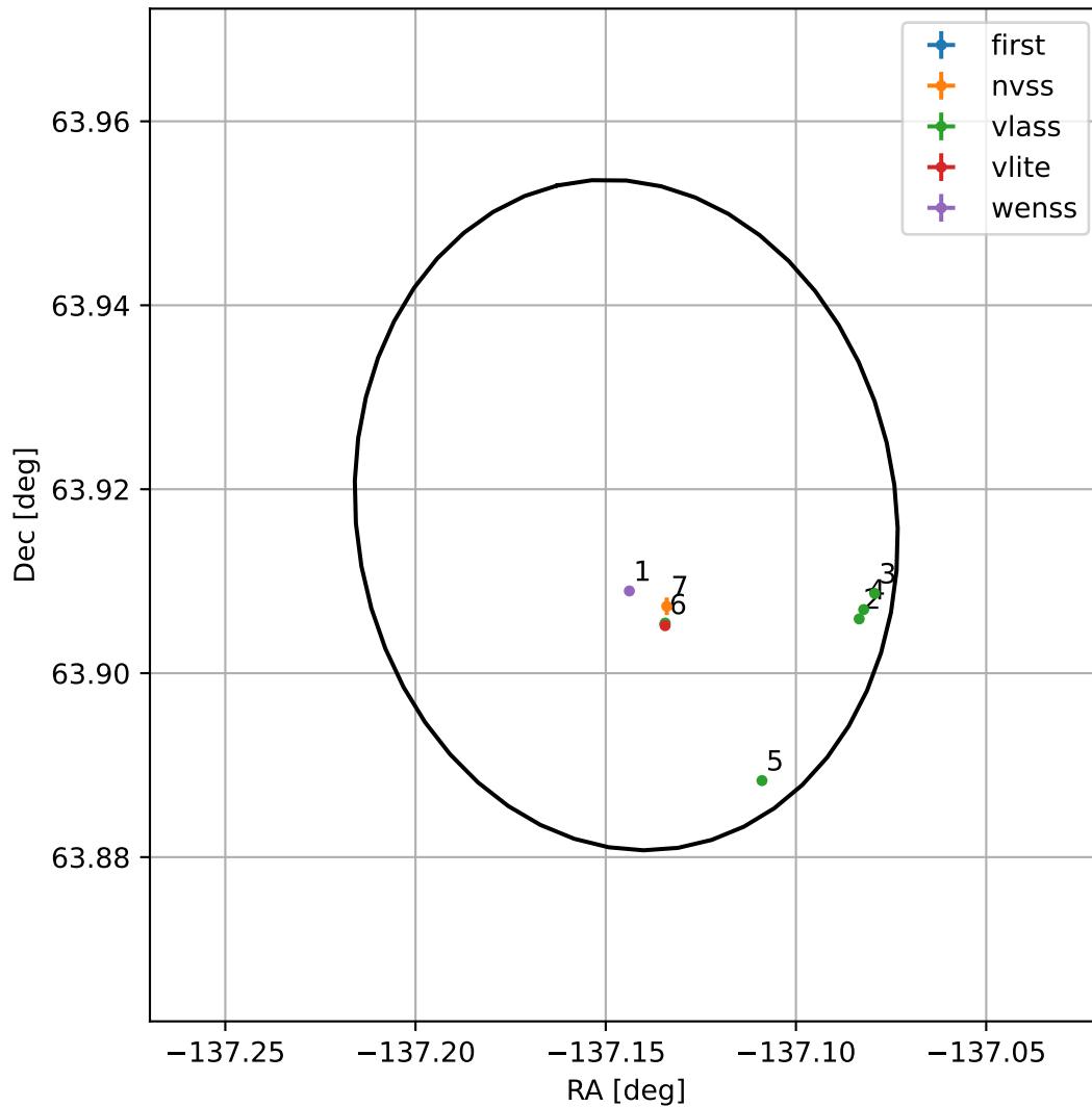
4FGL J1451.4+6355
