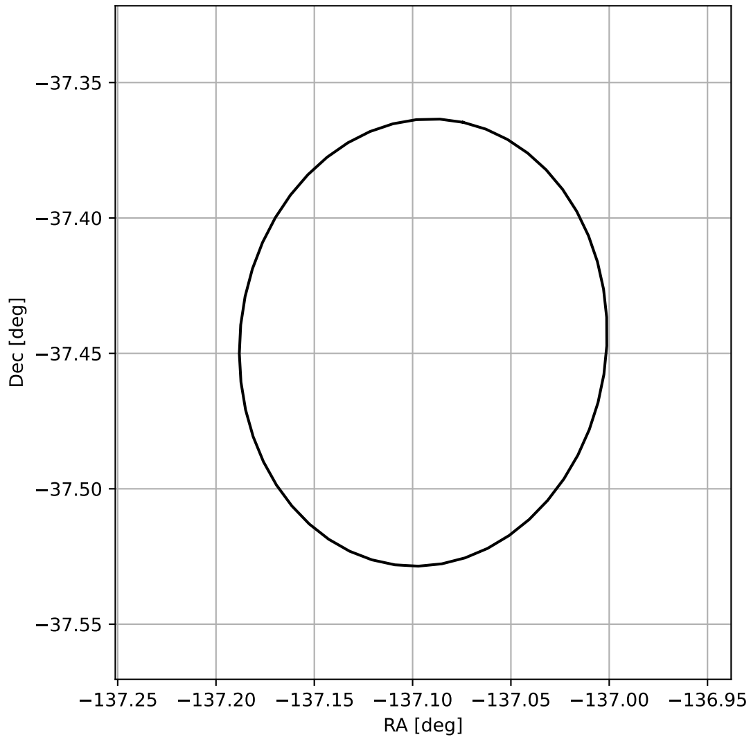
4FGL J1451.6-3726
