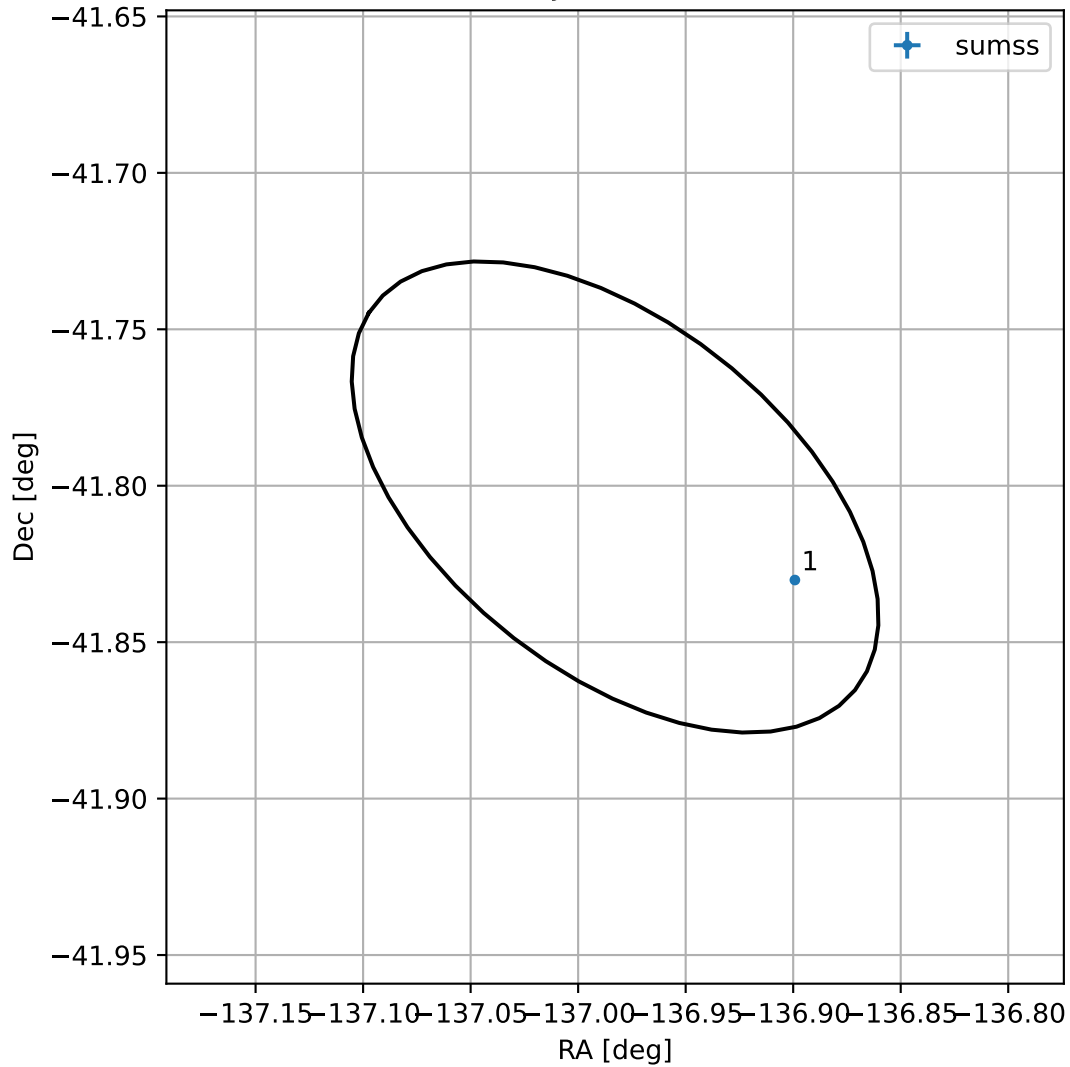
4FGL J1452.0-4148
